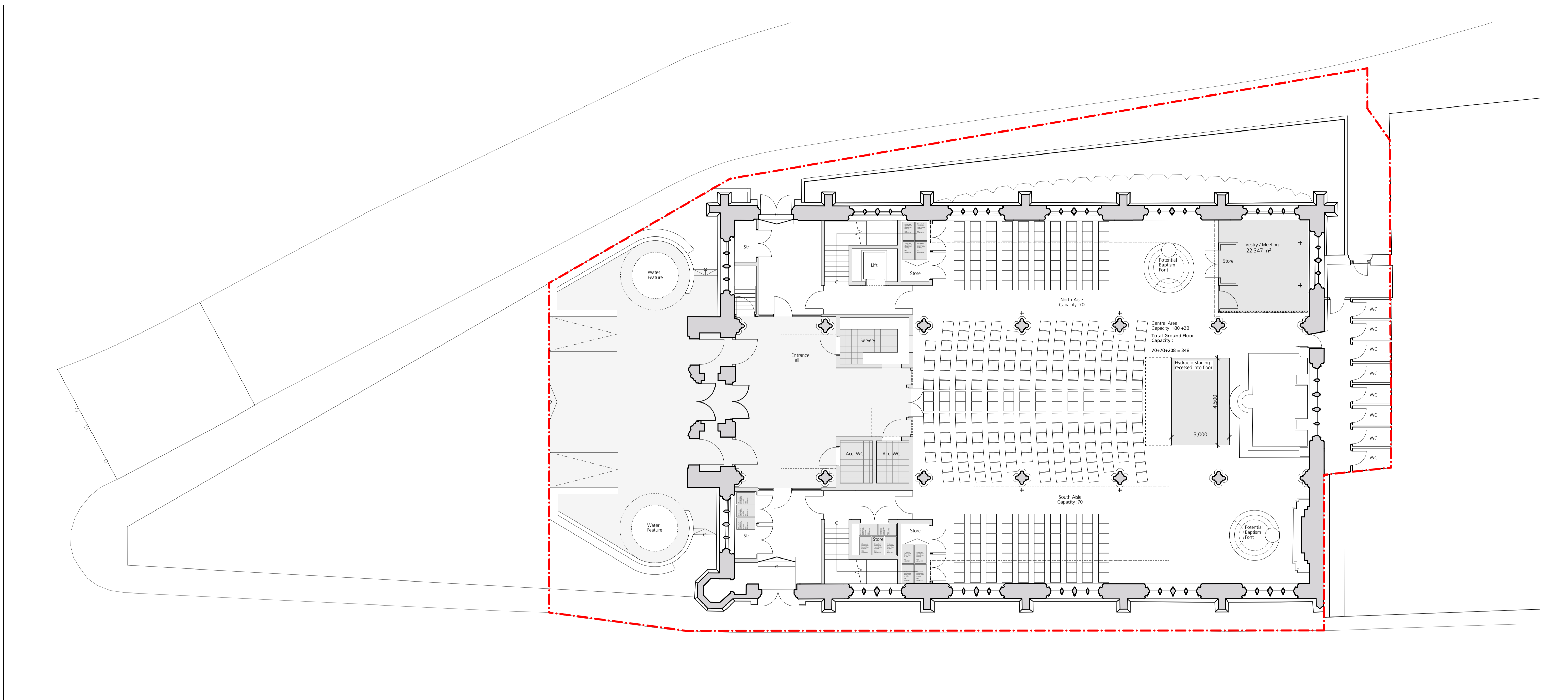
PROPOSED GROUND FLOOR PLAN 1:100 @ A1
